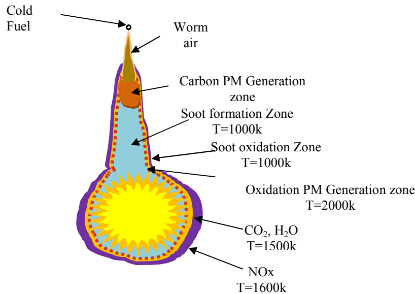
Figure 3 Diesel combustion process
