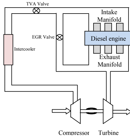
Figure 1 Diesel engine air circulation path
