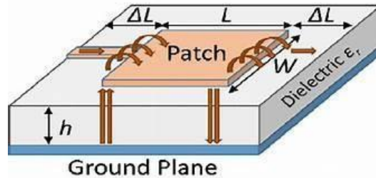
Fig 3.1 Microstrip patch
