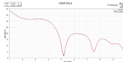
Fig 5.2 VSWR plot 5.2GHz Microstrip patch antenna
