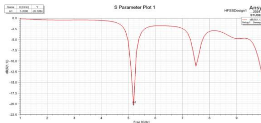
Fig 5.1 S parameter plot of 5.2GHz Microstrip patch antenna
