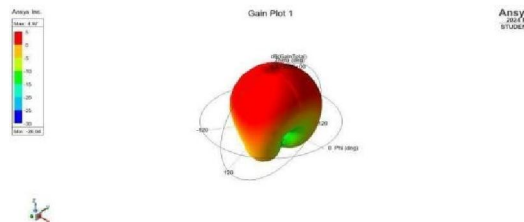
Fig 5.3 Gain plot 5.2GHz Microstrip patch antenna
