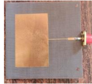
Fig 5.4 Fabricated Microstrip patch antenna
