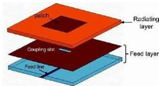
Fig 2.3 Feed layer
