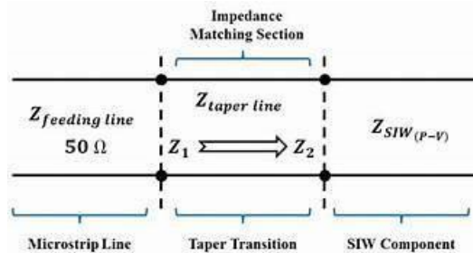
Fig 3.2 Impedance matching section
